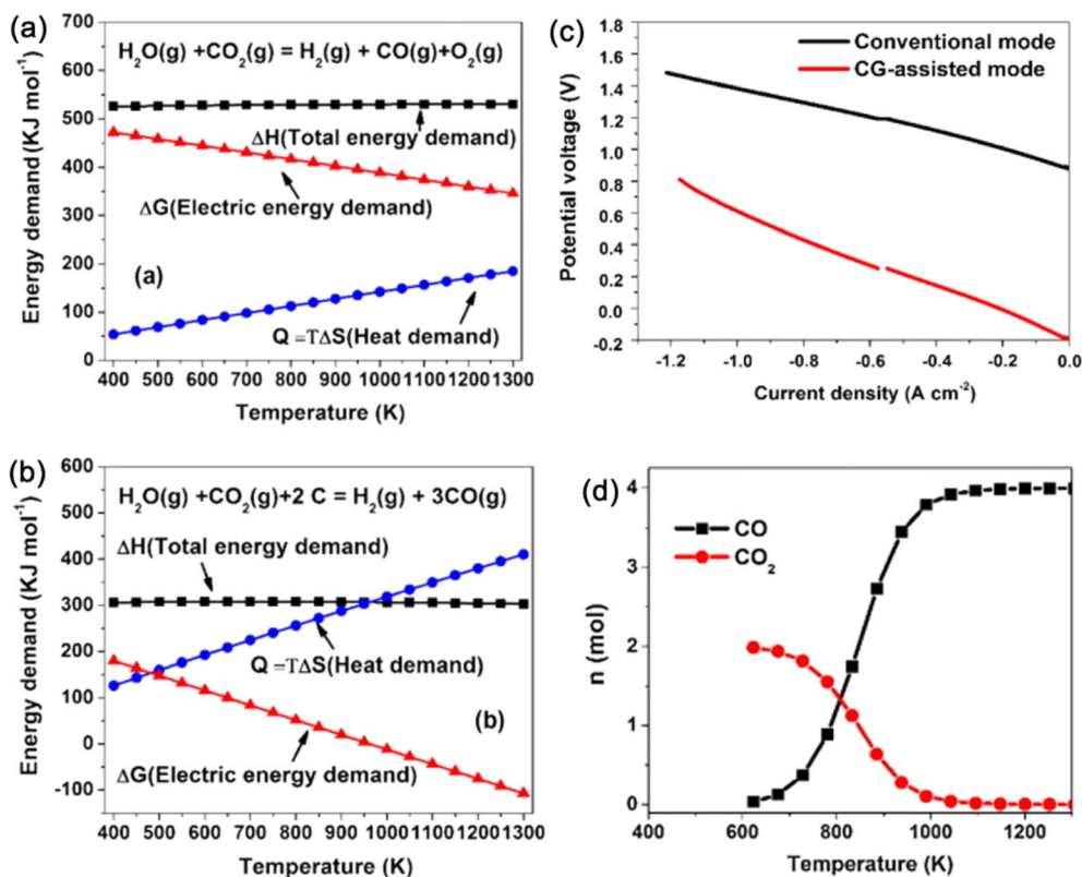
Fig. 4 Thermodynamic calculation of the required energy for \text{CO}_2-\text{H}_2\text{O} co-electrolysis without (a) and with (b) carbon fuel in the anode, (c) comparison of the I-V curves of the electrolysis cell, and (d) temperature-dependence of anode outlet gas composition. 138 Reproduced with permission.
