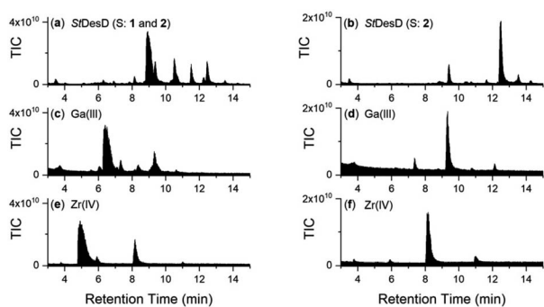
Fig. 4 LC-MS traces detected by TIC from the reaction solution of StDesD with MgCl 2 and ATP with substrate(s): (a) 1 and 2, and following the addition to (a) of (c) Ga(III) or (e) Zr(IV); or (b) 2 alone, and following the addition to (b) of (d) Ga(III) or (f) Zr(IV).
