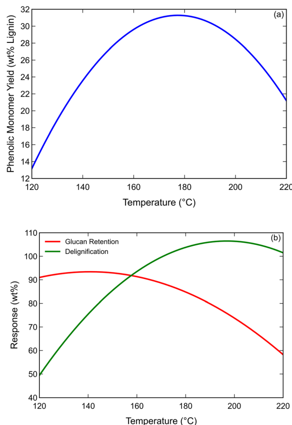
Fig. 3 Modelled univariate effect of reaction temperature on (a) phenolic monomer yield (b) glucan retention and delignification where other explanatory variables were constant at their center points (time: 32 min, O 2 pressure: 120 psi, catalyst: 19 wt%, NaOH: 1.25 M). Glucan retention is calculated based on the initial cellulose content of the biomass.
