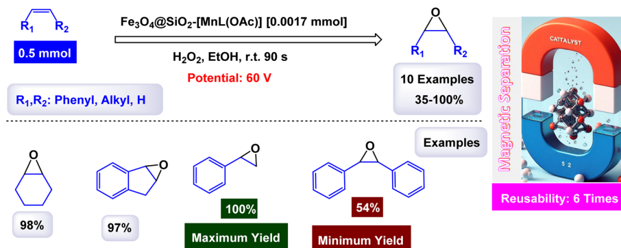
Scheme 8 Epoxidation of alkynes [catalysis by \text{Fe}_3\text{O}_4@\text{SiO}_2\text{-[MnL(OAc)]} nanocomposite].
