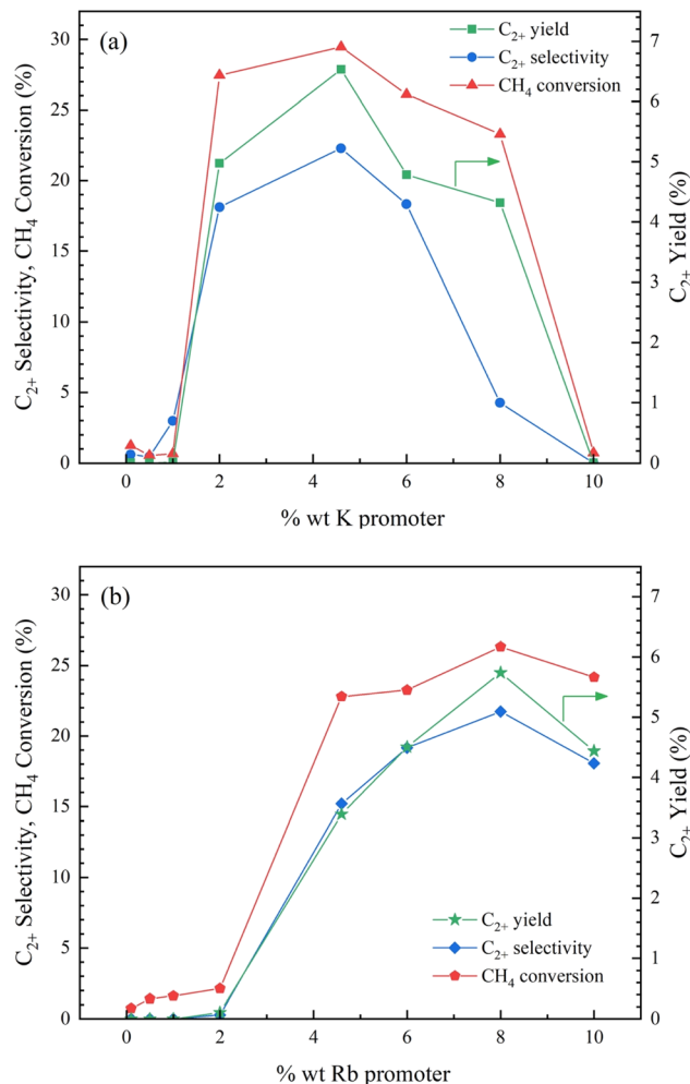
Fig. 10 Catalytic performance of (a) K- Co/Al_2O_3 catalyst and (b) Rb- Co/Al_2O_3 with varying weight percentages of promoter for OCM reaction. Reaction conditions: CH_4 : O_2 ratio = 2 : 1, catalyst weight = 40 mg, total feed flow rate = 40 mL\ min^{-1} , reactor temperature = 490 °C.
