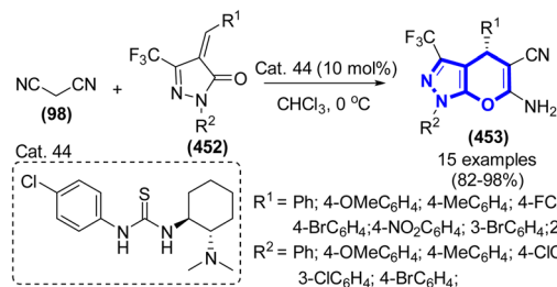
Scheme 121 Synthesis of functionalized dihydropyrano[2,3-c]pyrazoles catalyzed by Cat. 44.
