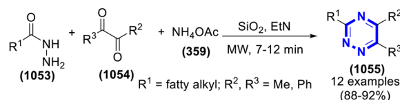
Scheme 293 Synthesis of 3,5,6-trisubstituted-1,2,4-triazines catalyzed by silica gel.
