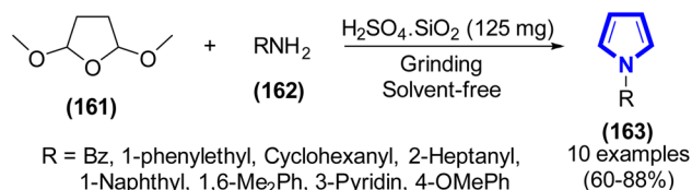
Scheme 44 Synthesis of N -substituted pyrroles catalyzed by \text{H}_2\text{SO}_4 \cdot \text{SiO}_2 (SSA).
