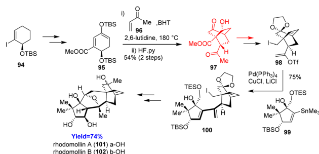
Scheme 13 Total syntheses of rhodomollins A ( 101 ) a-OH and rhodomollin B ( 102 ) b-OH. 43
