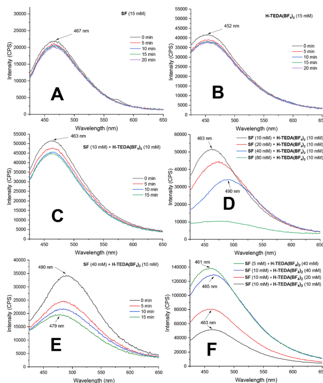
Fig. 2 Luminescence of SF and H-TEDA ( BF 4 ) 2 . (A) SF only (15 mM). (B) H-TEDA ( BF 4 ) 2 only (15 mM). (C) SF and H-TEDA ( BF 4 ) 2 in 1 : 1 ratio. (D) H-TEDA ( BF 4 ) 2 (10 mM) with increasing concentrations of SF . (E) SF and H-TEDA ( BF 4 ) 2 in a 4 : 1 ratio. (F) SF (10 mM) with increasing concentrations of H-TEDA ( BF 4 ) 2 .
