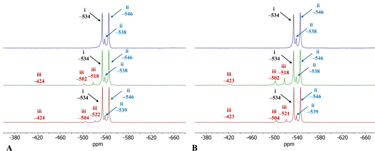
Fig. 4 ^{51}\text{V} NMR spectra measured at 37^\circ\text{C} after 42 h (A) and 7 d (B) of incubation of \text{Cs}_2[\text{V}_2\text{O}_4(\text{mal})_2]\cdot 2\text{H}_2\text{O} (5 mM) dissolved in \text{D}_2\text{O} (red lines); in 1.1 M sodium chloride, 0.1 M sodium acetate pH 4.0 and 10% \text{D}_2\text{O} (green lines); and in 1.1 M sodium chloride, 0.1 M sodium acetate pH 4.0 and 10% \text{D}_2\text{O} in presence of HEWL ( 13 \text{ mg mL}^{-1} ) (blue lines). "i" indicates [\text{V}_2\text{O}_4(\text{mal})_2]^{2-} , "ii" indicates [\text{V}_2\text{O}_5(\text{mal})]^{2-} and "iii" the decavanadate anion \text{V}_{10} .
