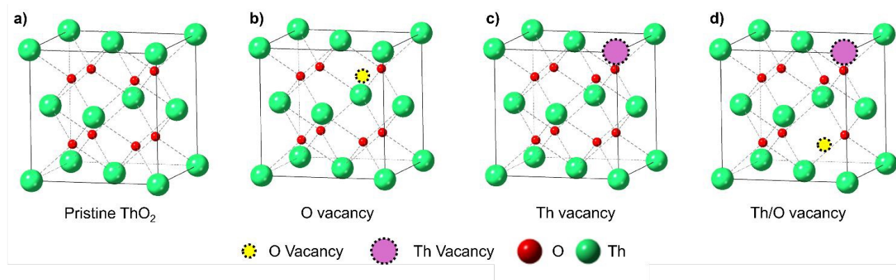
Figure 13. Modified figure from Park et al. , 224 shows the various defects in the \text{ThO}_2 unit cell.
