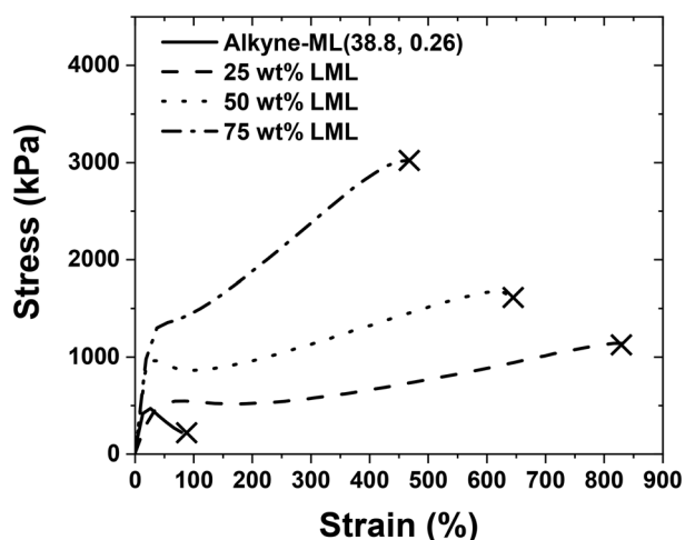
Fig. 6 Representative tensile data for alkyne-ML(38.8, 0.26) and LML/ML blends after solvent casting. Tensile tests were performed with an extension rate of 305 \text{mm min}^{-1} , with the break point indicated by x.
