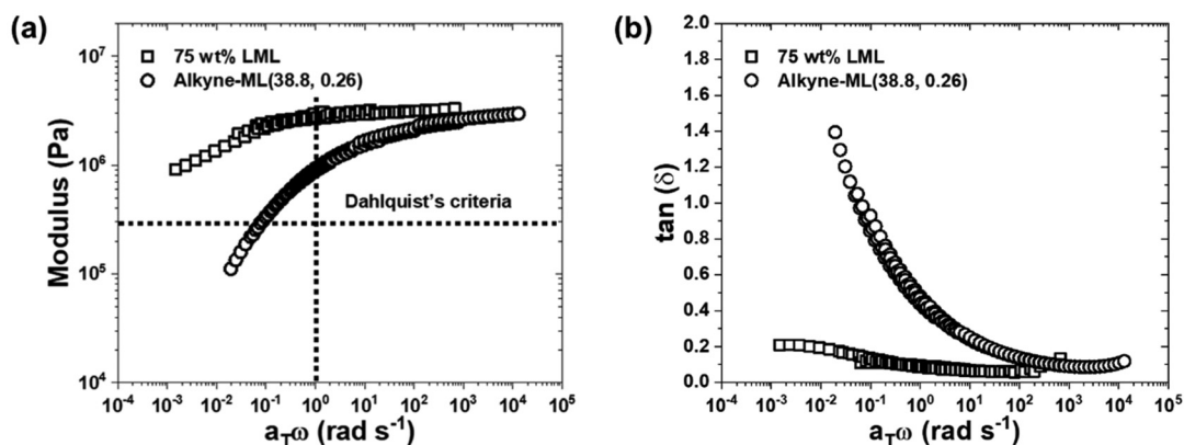
Fig. 5 Master curves for the (a) storage modulus ( G' ) and (b) \tan(\delta) of alkyne-ML(38.8, 0.26) and 75 wt% LML blends after solvent casting. The Dahlquist criterion ( G' = 0.3 MPa at 1 \text{rad s}^{-1} ) is marked by dashed lines.
