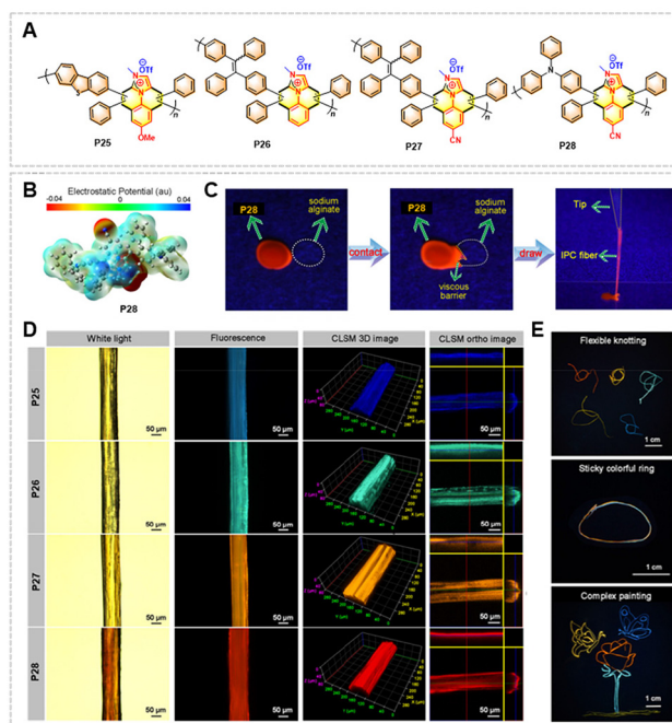
Fig. 11 (A) Structures of CMCPs (P25–P28). (B) Electrostatic potential surface of the repeating unit of P28. (C) Fluorescence photographs showing the IPC fiber drawing process under 365 nm UV irradiation. (D) Optical and fluorescence images of the freshly formed cationic CMCPs/sodium alginate fibers captured under white light and UV light irradiation (340–380 nm), respectively, using an inverted fluorescence microscope (the front two columns of images), and their fluorescence 3D images together with the corresponding cutaway view obtained by CLSM (the latter two columns of images). All colors are false colors in these images. (E) Diverse forms of the obtained fluorescent cationic polyelectrolyte/sodium alginate fibers. The macroscopic fluorescence images feature real colors and were directly captured using a digital camera under 365 nm UV light irradiation. Adapted with permission from ref. 8. Copyright 2023 American Chemical Society.
