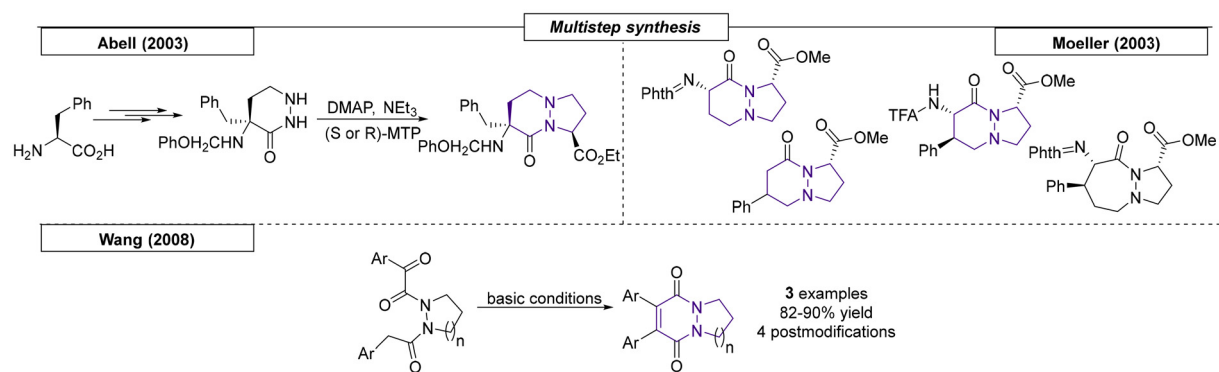
Scheme 44 Multistep synthetic procedures that produce pyrazolo-pyridazines.
