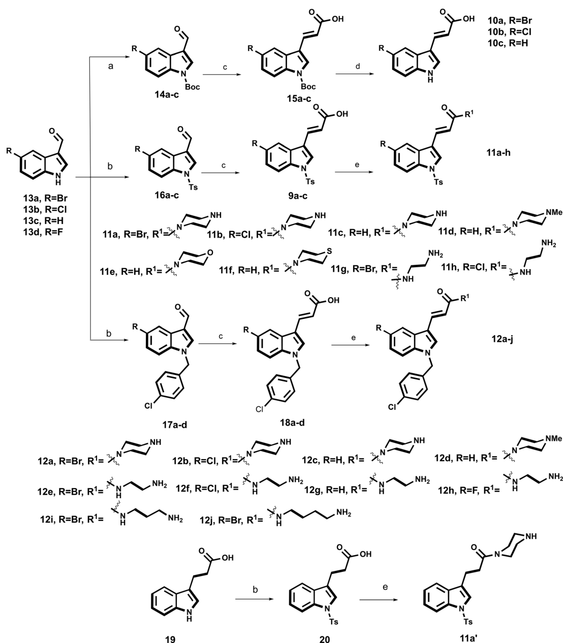
Scheme 1 Synthetic route for the indolyl acrylamides analogues 11a-h , 11a' and 12a-j . a) 13a-c , \text{Boc}_2\text{O} , NaH, THF, rt, 24 h; b) 13a-c , p -toluenesulfonyl chloride or p -chlorobenzyl chloride, NaOH, and TEBAC, DCM, rt, 16 h; c) 14a-c or 16a-c , malonic acid, piperidine, pyridine, 80 °C, 5 h; d) 15a-c , TFA, DCM, rt, 1 h; e) 9a-c or 18a-d , HBTU, DIPEA, DCM/DMF (3:1), rt, 5 h.
