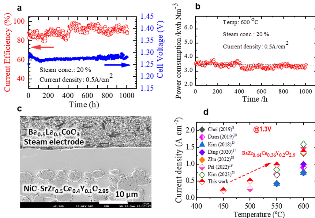
Fig. 6 (a) Long-term durability test of the BSZCY9144362-based cell at 600 °C. (b) Calculated amount of electricity to produce 1 N m³ of H₂ as a function of time. (c) Microstructure of cell post measurement. (d) Performance comparison of our BSZCY44362-based cell with similar electrolyte composition reported in the literature.
