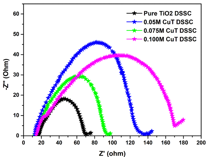
Fig. 11 EIS spectra of pure and various Cu-doped TiO 2 -based DSSCs.
