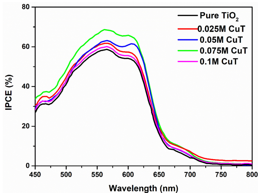
Fig. 10 IPCE spectra of pure and various Cu-doped TiO 2 -based DSSCs.
