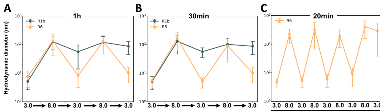
Fig. 7 Assays to study pH-responsive assembly kinetics of reflectins R1b and R6. Hydrodynamic diameter variations were measured by DLS after pH changes between 3.0 and 8.0. (A) R1b and R6 with 1-hour incubations. (B) R1b and R6 with 30-minute incubations. (C) R6 only, with 20-minute incubations over 8 pH cycles. Data points represent the mean value of measured hydrodynamic diameter \pm standard deviation of triplicate measurements for each sample.
