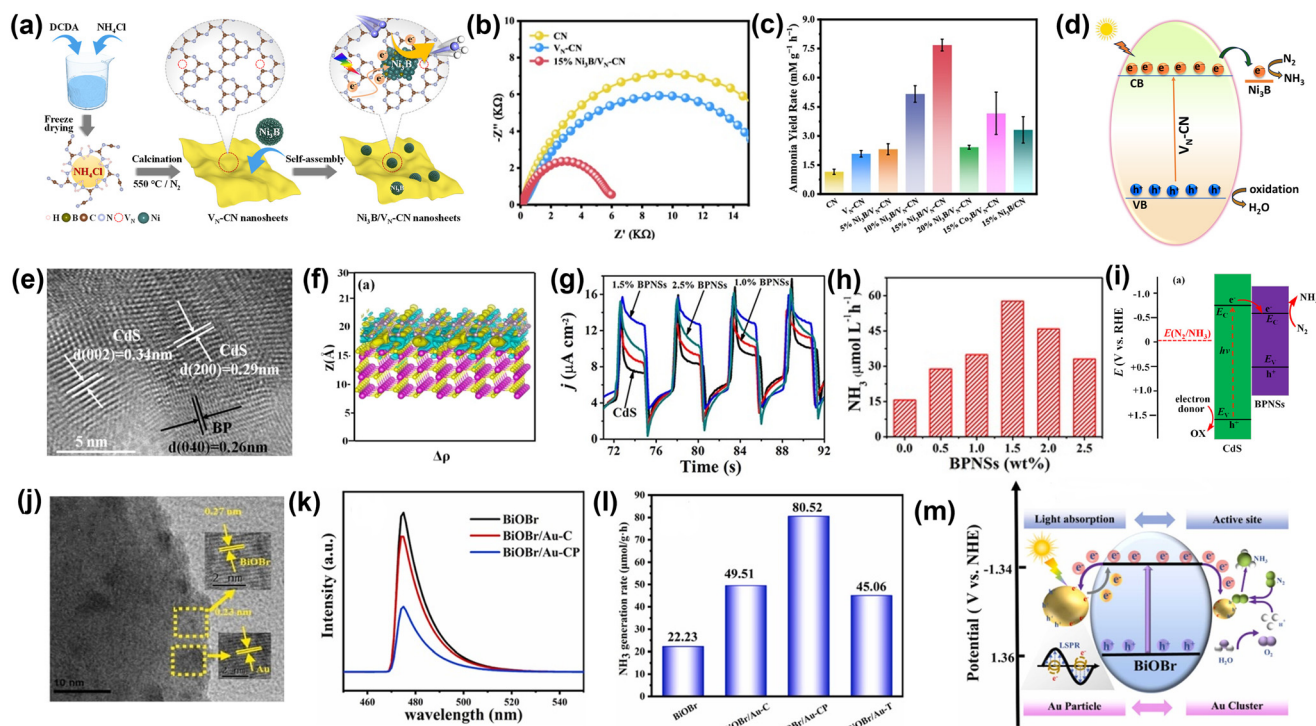
Fig. 13 (a) A schematic illustration depicts the formation process of the Ni 3 B/V N -CN photocatalyst. (b) Impedance plots of CN, V N -CN, and 15% Ni 3 B/V N -CN. (c) The ammonia yield of the synthesized samples is reported. (d) A possible mechanism for the photocatalytic NRR on the Ni 3 B/V N -CN photocatalyst is proposed. Reproduced from ref. 109 with permission from [American Chemical Society], copyright [2023]. (e) HRTEM images of 1.5% BPNS/CdS photocatalyst. (f) The charge density difference at the BPNS/CdS heterojunction interfaces are shown, with the yellow and blue isosurfaces representing electron gain and loss, respectively. (g) The time-dependent photocurrent response of different BPNS/CdS samples and bare CdS is examined. (h) The NH 3 formation rates of different samples are compared. (i) A proposed photocatalytic mechanism for efficient nitrogen fixation on BPNS/CdS photocatalysts is presented. Reproduced from ref. 110 with permission from [American Chemical Society], copyright [2020]. (j) HRTEM images of BiOBr/Au-CP. (k) PL spectra and (l) NH 3 yield rates of BiOBr, BiOBr/Au-C, BiOBr/Au-CP, and BiOBr/Au-T. (m) The mechanism of internal charge transfer and photocatalytic nitrogen fixation in BiOBr/Au-CP. Reproduced from ref. 111 with permission from [Elsevier], copyright [2023].
