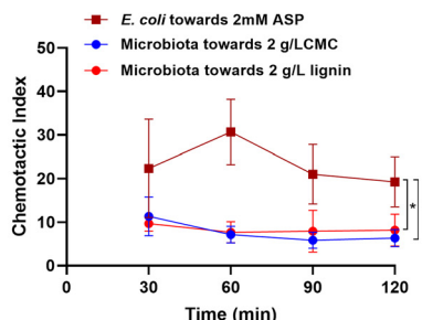
Fig. 5 Studying the relationship between chemotaxis and degradation using a leaf mould microbiota. (a) The process of identifying the link between bacterial chemotaxis and degradation of CMC or alkali lignin, and the chemotactic-based sorting of cellulolytic bacteria. (b) Bacteria from the microbiota showed strong chemotaxis towards CMC ( 2 \text{ g L}^{-1} in CB) and alkali lignin ( 1 \text{ g L}^{-1} in CB) compared with the control (filled with CB in a chemoattractant reservoir). Shaded regions indicate standard deviations. (c) The chemotaxis index of bacteria towards different compounds. Data of E. coli towards 2 mM ASP were derived from Fig. 3c. (d) Chemotactic bacteria were sorted and retrieved off-chip after 2 hours of assays. Each 100 \mu\text{L} bacterial suspension was spread on TSB agar for total cultivable cell number counting, on CMC selective agar for isolating cellulolytic bacteria, and on alkali lignin selective agar for isolating lignin-degradation bacteria respectively. CB: chemotaxis buffer. CMC: sodium carboxymethyl cellulose. (** p < 0.01 , * p < 0.05 , unpaired one-tailed t-test).
