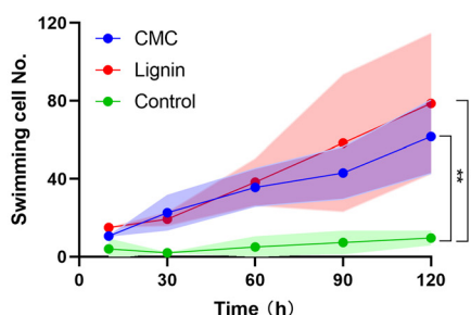
Fig. 5 Studying the relationship between chemotaxis and degradation using a leaf mould microbiota. (a) The process of identifying the link between bacterial chemotaxis and degradation of CMC or alkali lignin, and the chemotactic-based sorting of cellulolytic bacteria. (b) Bacteria from the microbiota showed strong chemotaxis towards CMC ( 2 \text{ g L}^{-1} in CB) and alkali lignin ( 1 \text{ g L}^{-1} in CB) compared with the control (filled with CB in a chemoattractant reservoir). Shaded regions indicate standard deviations. (c) The chemotaxis index of bacteria towards different compounds. Data of E. coli towards 2 mM ASP were derived from Fig. 3c. (d) Chemotactic bacteria were sorted and retrieved off-chip after 2 hours of assays. Each 100 \mu\text{L} bacterial suspension was spread on TSB agar for total cultivable cell number counting, on CMC selective agar for isolating cellulolytic bacteria, and on alkali lignin selective agar for isolating lignin-degradation bacteria respectively. CB: chemotaxis buffer. CMC: sodium carboxymethyl cellulose. (** p < 0.01 , * p < 0.05 , unpaired one-tailed t-test).
