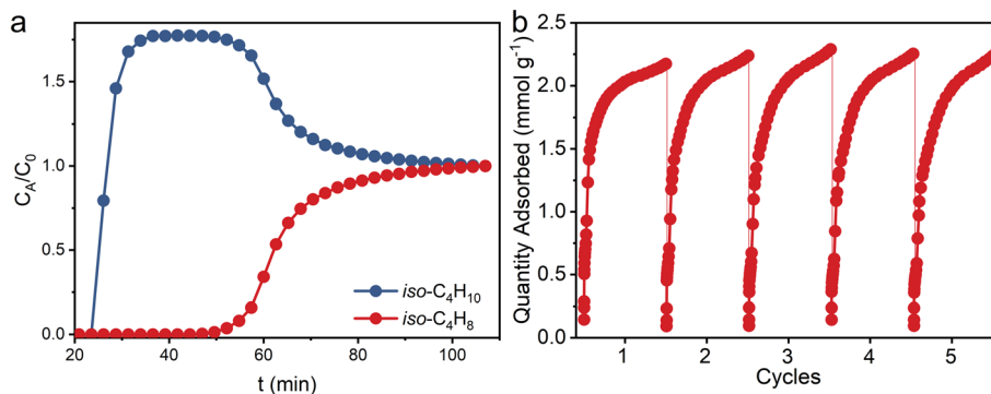
Fig. 4 (a) Breakthrough experiment on ZU-603 using a gas mixture of iso- \text{C}_4\text{H}_8 /iso- \text{C}_4\text{H}_{10} (50/50, v/v) with a mix gas flow rate of 0.8 mL min -1 at 298 K and (b) cycling adsorption tests of iso- \text{C}_4\text{H}_8 on ZU-603 at 298 K.
