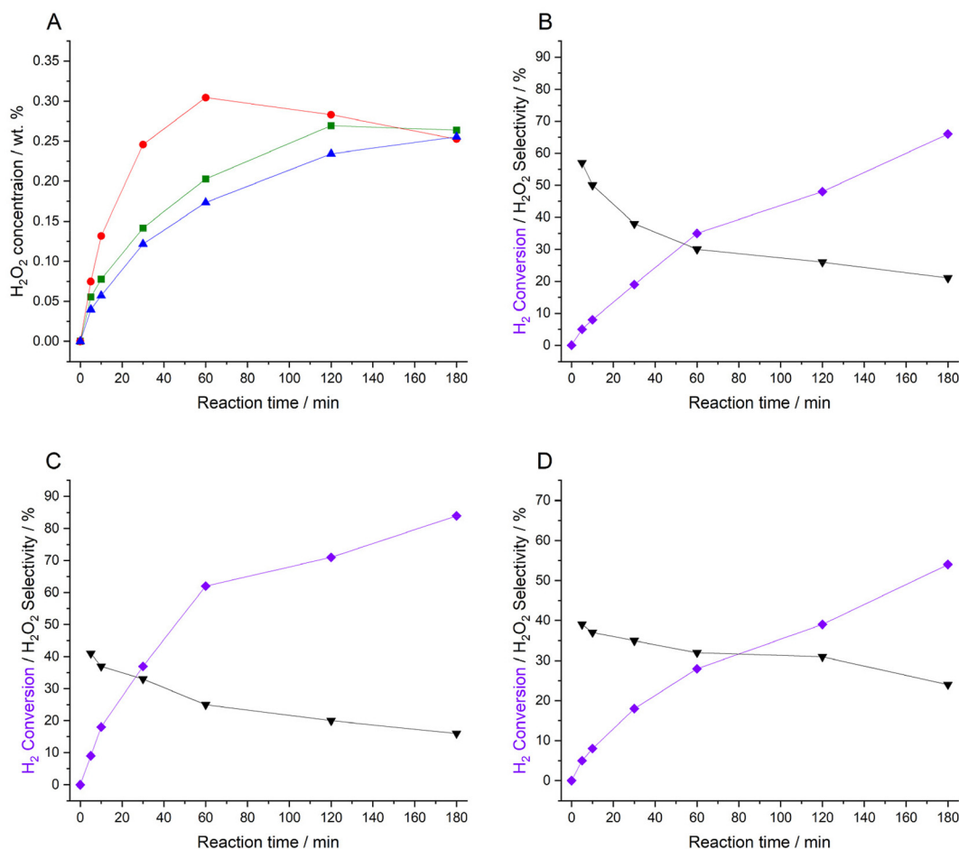
Fig. 5 Comparison of catalytic activity towards the direct synthesis of \text{H}_2\text{O}_2 , as a function of reaction time. (A) Catalytic activity based on net \text{H}_2\text{O}_2 concentration. Determination of \text{H}_2 conversion and \text{H}_2\text{O}_2 selectivity for the (B) 0.5\%\text{Au}-0.5\%\text{Pd}/\text{TiO}_2 (C) 0.5\%\text{Au}-0.5\%\text{Pd}-0.02\%\text{Fe}/\text{TiO}_2 and (D) 0.5\%\text{Au}-0.5\%\text{Pd}-1.0\%\text{Fe}/\text{TiO}_2 catalysts. Key: 0.5\%\text{Au}-0.5\%\text{Pd}/\text{TiO}_2 (green squares), 0.5\%\text{Au}-0.5\%\text{Pd}-0.02\%\text{Fe}/\text{TiO}_2 (red circles), 0.5\%\text{Au}-0.5\%\text{Pd}-1.0\%\text{Fe}/\text{TiO}_2 catalysts (blue triangles). \text{H}_2 conversion (purple diamonds), \text{H}_2\text{O}_2 selectivity (black inverted triangles). \text{H}_2\text{O}_2 direct synthesis reaction conditions: catalyst (0.01 g), \text{H}_2\text{O} (2.9 g), MeOH (5.6 g), 5% \text{H}_2/\text{CO}_2 (420 psi), 25% \text{O}_2/\text{CO}_2 (160 psi), 2^\circ\text{C} , 1200 rpm.
