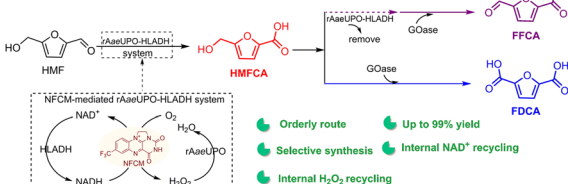
Scheme 1 The previous and current strategies for the selective synthesis of HMFA, FFCA and FDCA. (A) Previous study. (B) This work.
