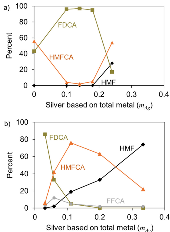
Fig. 7 Effect of silver loading on a bimetallic (a) Au/Ag SiO 2 catalyst (conditions: 79:1 HMF:Ag molar ratio, 0.4 mmol NaHCO 3 , T = 353 K, P_{O_2} = 1 MPa, and t = 6 h) 68 and (b) Pt/Ag catalyst where the x-axis represents the mass fraction of Ag of the total mass of the metals. Reaction conditions: 50:1 HMF:Pt molar ratio, 0.8 mmol NaHCO 3 , T = 373 K, O 2 bubbling at 75 mL min -1 , and t = 1 h. 60
