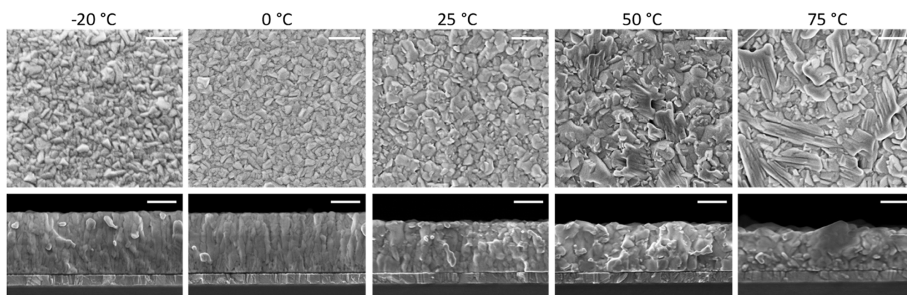
Fig. 2 Surface morphology and cross-section SEM images of a series of perovskite films deposited at increasing substrate temperature as noted above. The scale bar corresponds to 300 nm.
