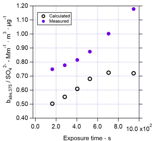
Fig. 4 Example of absorption coefficients (units of Mm^{-1} ) at 375 nm, with normalization by sulfate AMS loading (units of \mu\text{g m}^{-3} ) at RH = 25\% \pm 5\% , for the data in Fig. 2 and 3. The measured values were obtained from the aethalometer. The predicted values arise from the measurements of mass loading of NVA in the flow tube and the measured MAC value for NVA.
