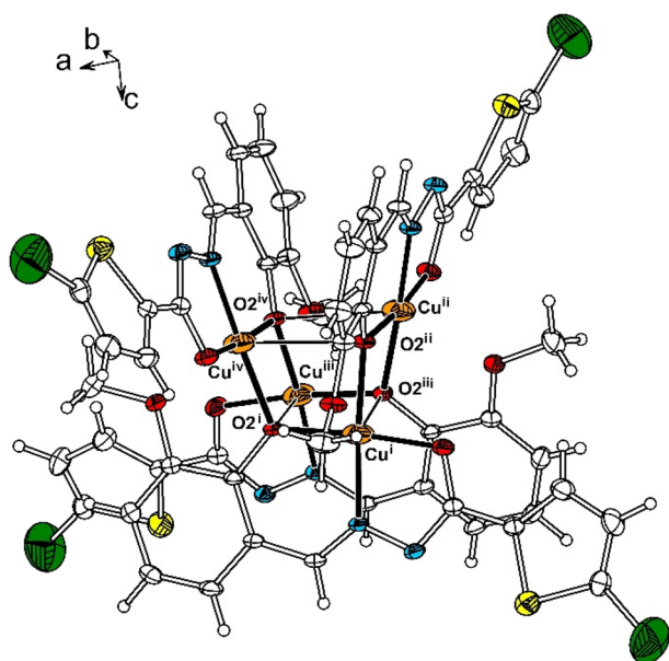
Fig. 3 View of the \text{Cu}_4\text{L}_4 complex. For clarity, only the symmetry-related copper and bridging hydroxyl oxygen atoms are labelled. Stronger coordination bonds are in full lines and weaker Cu-ligand contacts in thin lines. Chlorine, sulphur, oxygen, and nitrogen atoms are, respectively, indicated in green, yellow, red and blue coloured ellipsoids. S_4 site-symmetry operations: (i) x, y, z ; (ii) -1/4 + y, 1/4 - x, 1/4 - z ; (iii) -x, 1/2 - y, z ; and (iv) 1/4 - y, 1/4 + x, 1/4 - z .
