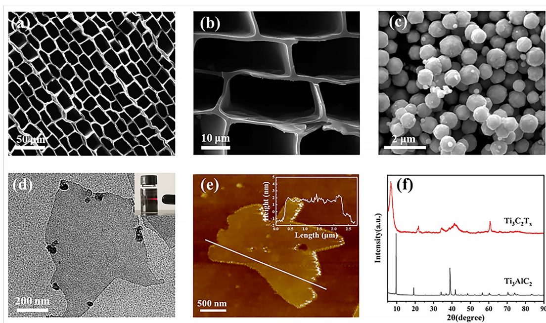
Fig. 2 SEM images of (a) cross-sectional wood, (b) high-magnification cross-sectional wood, and (c) CoNi. (d) TEM image of \text{Ti}_3\text{C}_2\text{T}_x MXene. (e) AFM image of \text{Ti}_3\text{C}_2\text{T}_x MXene. (f) XRD patterns of \text{Ti}_3\text{AlC}_2 and \text{Ti}_3\text{C}_2\text{T}_x MXene.
