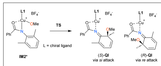
methoxycopper(III) IM2 is larger than that of Cu(I) IM2' with the nitrenium moiety (see the ESI†). In addition, the calculations suggest that the C–O bond-forming process through TS 2-3 is the rate-determining process, the activation energy of which is calculated to be 25.6 kcal mol -1 . It should be noted that the methoxy group preferentially migrates to the methyl-bound ortho position, where the nucleophilic attack on the ortho carbon with a methyl substituent is energetically favored over
