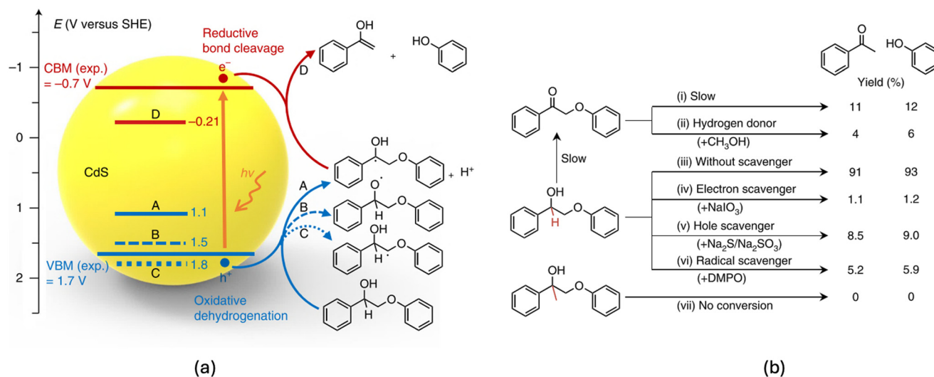
Scheme 2 (a) Proposed electron-hole coupled (EHCO) mechanism for CdS-catalysed C_\beta -O bond cleavage of a dimeric \beta -O-4 lignin model compound through a C_\alpha radical intermediate; (b) the control experiments with various reactants or additives (this scheme has been reproduced from ref. 22 with permission from Nature Publication Group, copyright 2018).
