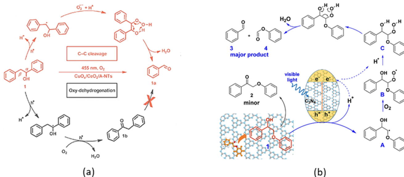
Scheme 12 The proposed reaction mechanism for photocatalytic cleavage of the \text{C}_\alpha - \text{C}_\beta bond in the (a) \beta -1 lignin model compounds over the \text{CuO}_x/\text{CeO}_2/\text{TiO}_2 catalyst and (b) in the \beta -O-4 lignin model compounds over mpg- \text{C}_3\text{N}_4 catalysts (this scheme is reproduced from ref. 66 and 88 with permission from American Chemical Society, copyright 2017 & copyright 2018).
