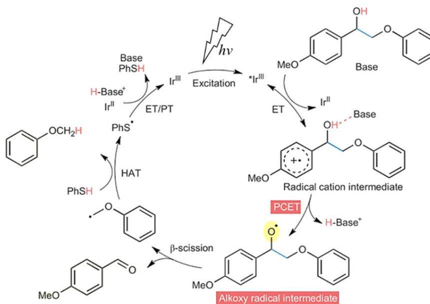
Scheme 10 Proposed reaction mechanism of \text{C}_\alpha\text{--C}_\beta bond cleavage by the Ir complex via a PCET process (this scheme has been reproduced from ref. 82 with permission from Elsevier, copyright 2019).
