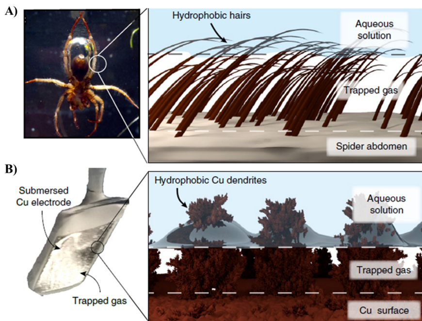
Fig. 13 (A) Diving bell spider for subaquatic breathing in and (B) on a hydrophobic dendritic Cu surface for aqueous \text{CO}_2 reduction. 178
