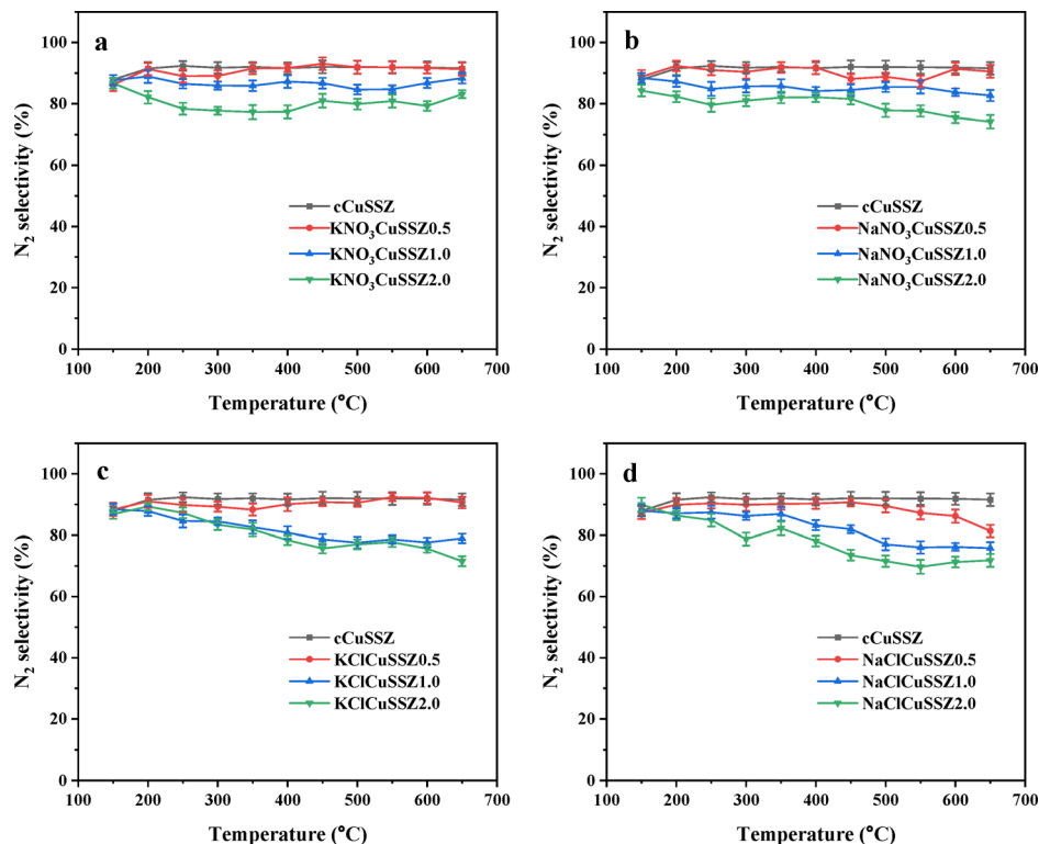
Fig. 2 Comparison of N_2 selectivity of the pristine cCuSSZ with the alkali metal poisoned Cu-SSZ-13 catalysts: (a) KNO_3 poisoned catalysts, (b) NaNO_3 poisoned catalysts, (c) KCl poisoned catalysts and (d) NaCl poisoned catalysts. Reaction conditions: 500 ppm NO, 500 ppm NH_3 , 5% O_2 and 3% H_2O in Ar balance; total flow rate: 200\text{ mL min}^{-1} ; atmospheric pressure.
