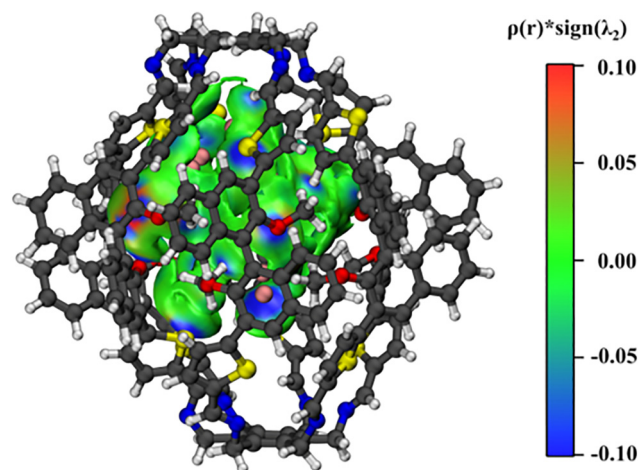
Fig. 4 The independent gradient model (IGM) isosurface (0.005 a.u.), colored in the -0.10 a.u. < \text{sign}(\lambda_2)\rho < +0.10 a.u. range for the \text{Au}_{18}-\mathbf{1} interaction in \text{Au}_{18}@\mathbf{1} . Blue/red accounts for stabilizing/destabilizing non-covalent interactions, whereas green isosurfaces denote London-type interactions.
