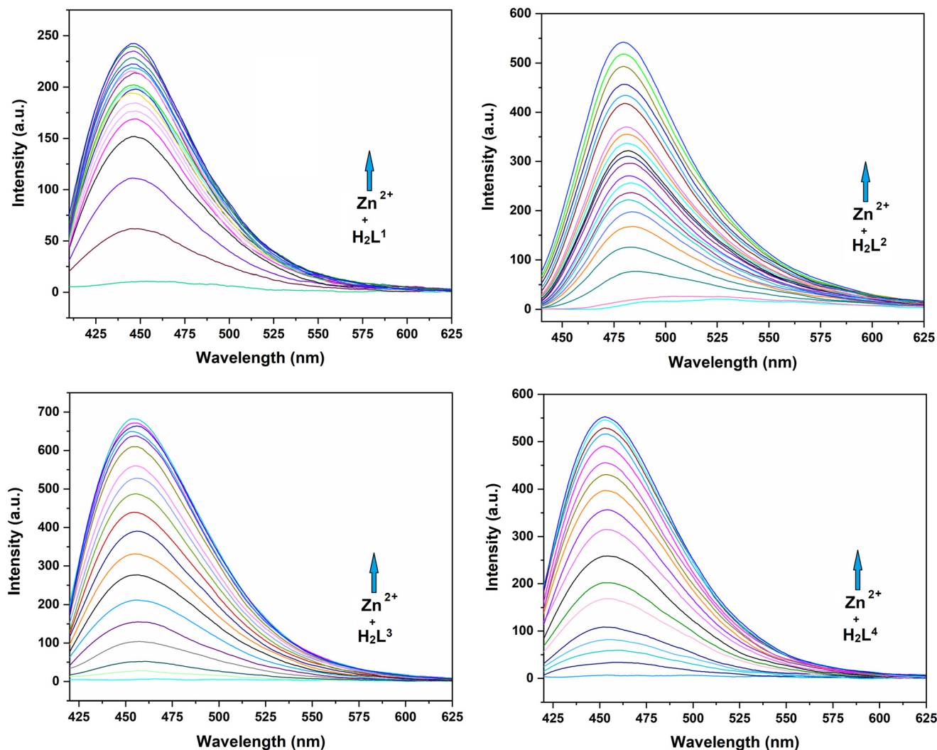
Fig. 11 Emission spectra of 10^{-3} M Schiff base ligands {H 2 L 1 (excitation 397 nm, 446 nm) or H 2 L 2 (excitation 419 nm, emission 479 nm) or H 2 L 3 (excitation 397 nm, emission 454 nm) or H 2 L 4 (excitation 397 nm, 453 nm)} in the presence of increasing concentration of free Zn 2+ ions at room temperature.
