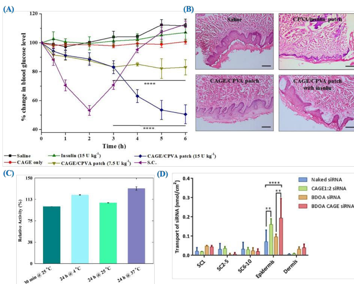
Fig. 5 (A) In vivo pharmacodynamic efficacy of CAGE/insulin administered in the buccal cavity of rats. (B) Hematoxylin and eosin (H&E) staining of rat buccal mucosa (scale bar= 200 μm). Figure reproduced with permission from ref 76. (C) Lysozyme relative activity under different incubation conditions. Figure reproduced with permission from ref 92. (D) Penetration of siRNA-ILs: porcine skin quantification using tape-stripping indicated improved permeation of robed-siRNA in presence of an IL (CAGE) into the epidermis. Figure reproduced with permission from ref 93.
