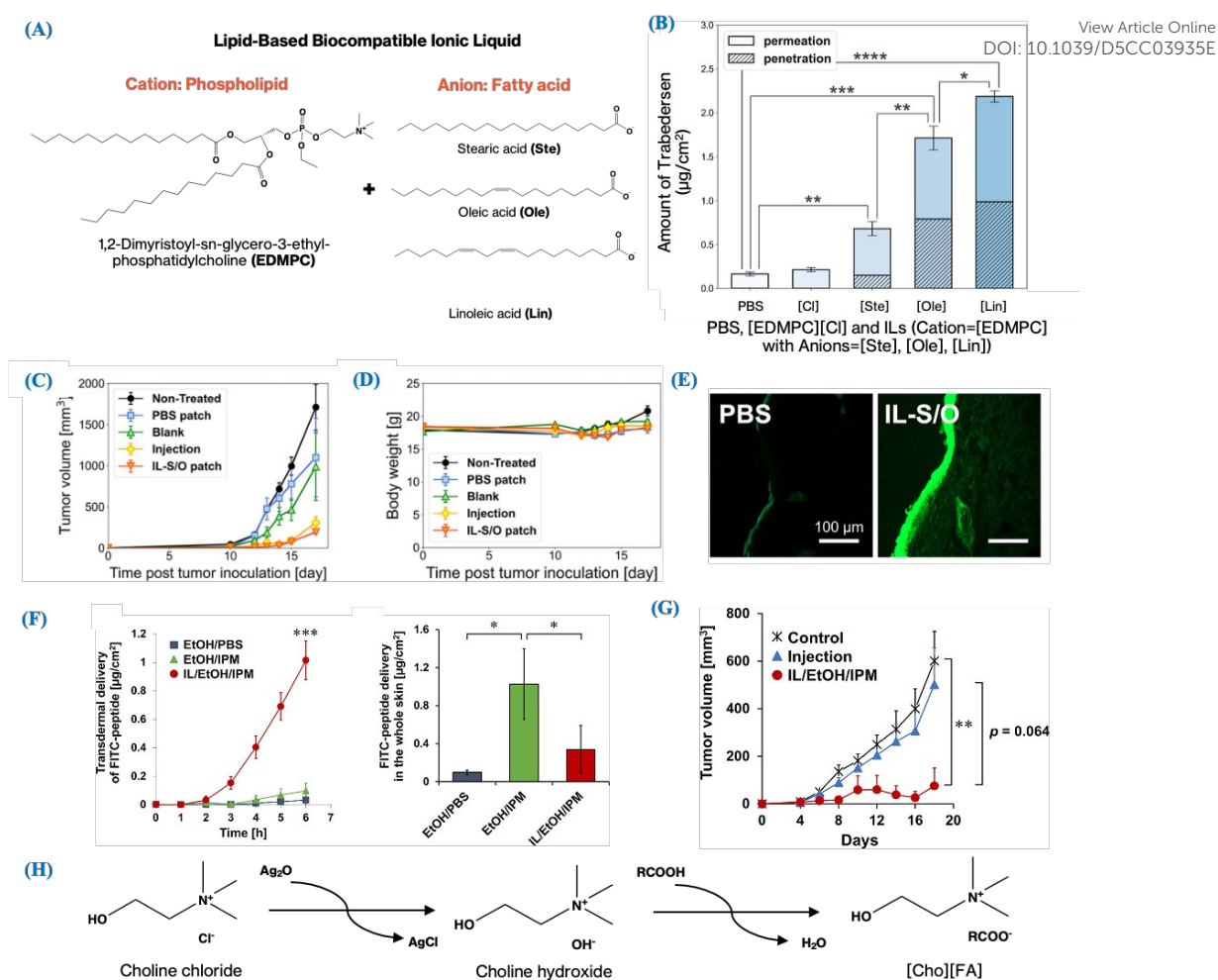
Fig. 7 (A) Chemical structures of cation and anions of lipid-based ILs. (B) Amount of trabectedin that permeated into the mouse skin and penetrated to the receiver phase. (C, D) Antitumor effect of trabectedin against B16F10 melanoma, (C) change in tumor volume and (D) change in body weight. (E) CLSM images of the skin cross sections of mouse skin treated with 6-carboxyfluorescein (FAM)-trabectedin in PBS or [EDMPC][Lin]-S/O. Scale bars: 100 \mu\text{m} . Figure reproduced with permission from ref 86. (F) Transdermal and topical delivery of FITC-peptide in EtOH/isopropyl myristate (IPM), EtOH/PBS, and IL/EtOH/IPM through the mouse skin. (G) Effect of transcutaneous cancer vaccination via the IL/EtOH/IPM system. (H) Synthetic scheme for [Cho][FA]. [Cho][FA] was synthesized through the metathesis reaction of choline chloride with \text{Ag}_2\text{O} to prepare choline hydroxide, followed by the acid-base neutralization reaction of the fatty acid and choline hydroxide. Figure reproduced with permission from ref 97.
