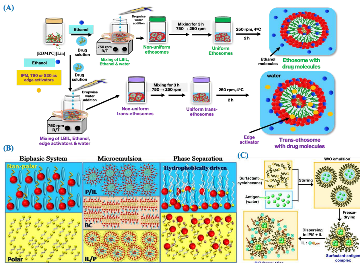
Fig. 4 Different types of IL-mediated formulations. (A) IL-mediated nanovesicular ETs. Figure reproduced with permission from ref 32. Copyright 2024. (B) IL-mediated MEs, P indicates polar. Figure reproduced with permission from ref 78. Copyright 2018. (C) IL-mediated solid in oil (S/O) dispersion, Figure reproduced with permission from ref 79. Copyright 2015.
