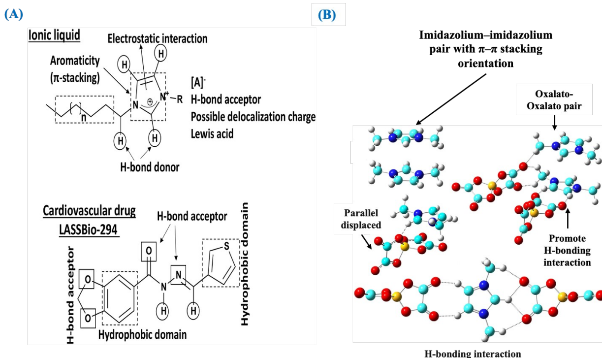
Fig. 3 (A) Schematic diagram of hypothetical interactions between imidazolium-based ILs and LASSBio-294, reproduced with permission from ref 51. (B) Representative molecular distributions among close-contact ionic groups showing \pi - \pi stacking orientation, reproduced with permission from ref 71. Copyright © 2017, American Chemical Society.
