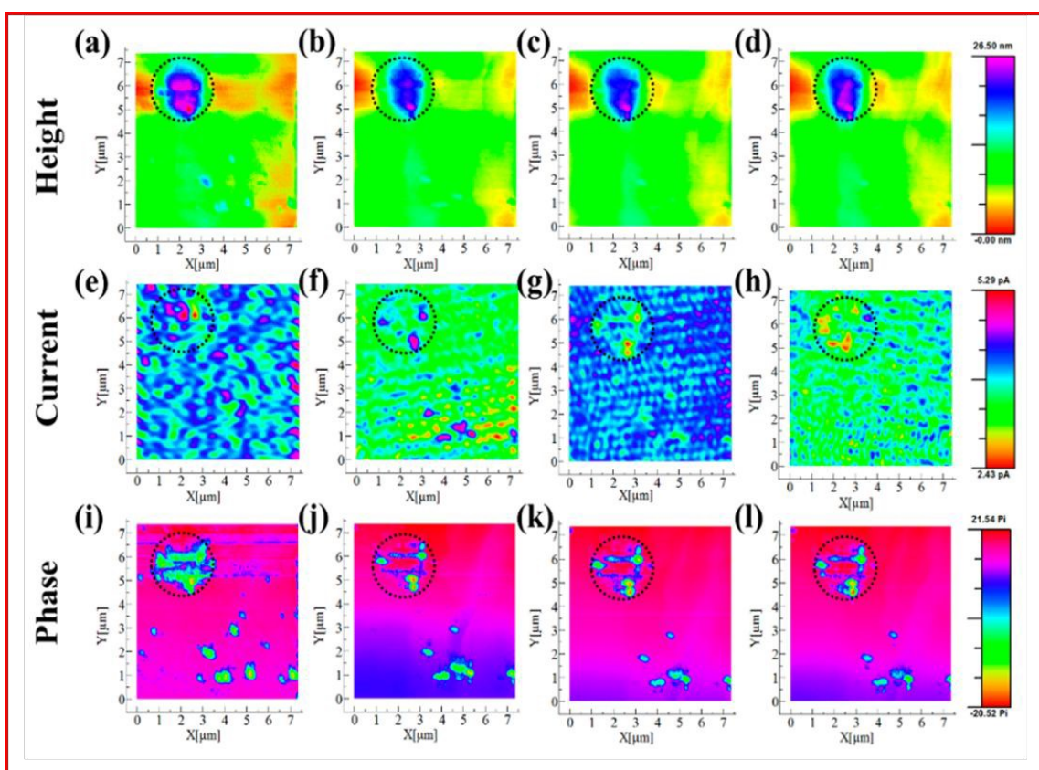
Fig. 12 AFM-SECM images of insoluble \text{Li}_2\text{S}/\text{Li}_2\text{S}_2 on the cathode. Simultaneously obtained data for the height (a-d), current (e-h) and phase shift (i-l) mapping are shown for samples before oxidation (a,e,i), at 2.5 V (b,f,j), 2.6 V (c,g,k) and 2.7 V (d,h,l) vs \text{Li}/\text{Li}^+ . ((a-l) Reproduced with permission from ref. 132, Copyright (2019) American Chemical Society).
