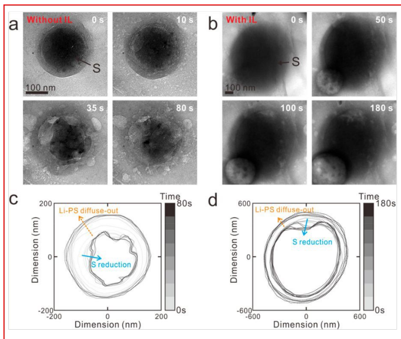
Fig. 14 (a-b) TEM image of sulfur nanoparticles during lithiation (a) without an ionic liquid electrolyte and (b) with ionic liquid electrolyte; (c-d) Outer boundaries of sulfur particle and LiPS and their evolution over time from (a) and (b) respectively. ((a-d) Reproduced with permission from ref. 140, Copyright (2020) American Chemical Society).
