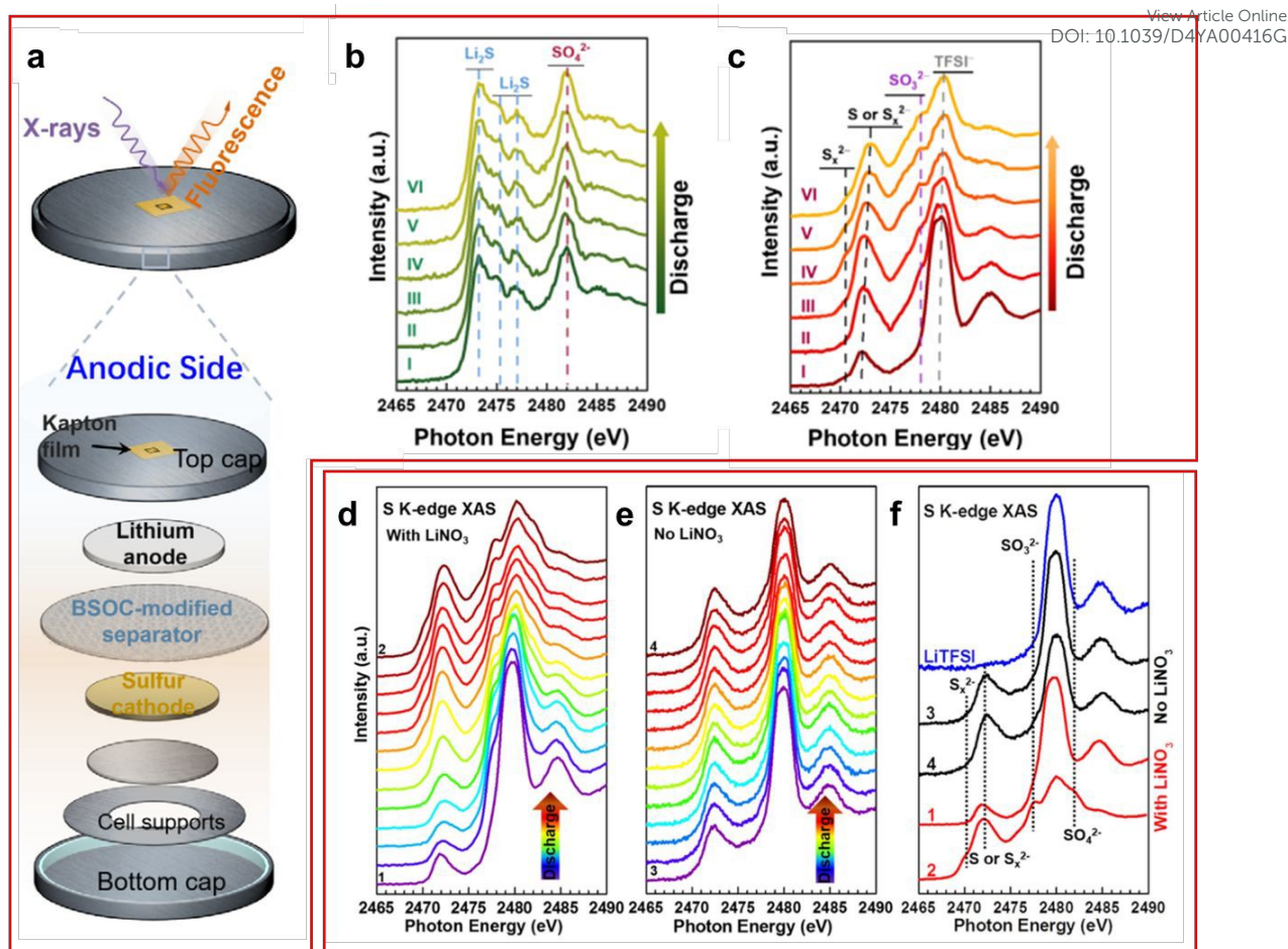
Fig. 6 (a) Schematic of a XAS cell used for operando studies of an LSB; (b-c) Operando XAS spectra of Jia et al. cell using (b) a bare PP separator and (c) a bismuth coated separator; (d-f) Operando XAS spectra for a cell (d) with \text{LiNO}_3 additive, (e) without \text{LiNO}_3 and (f) a comparison of the spectra at full charge and discharge for both conditions with LiTFSI spectrum as reference. ((a-c) Reproduced with permission from ref. 79, Copyright (2021) Wiley-VCH; (d-f) Reproduced with permission from ref. 15, Copyright (2018) Elsevier).
