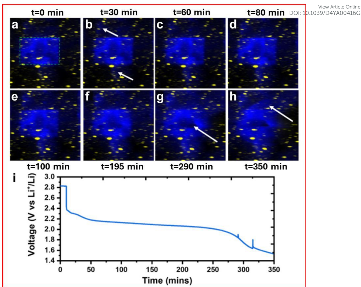
Fig. 10 (a-h) XRF map of a LSB with sulfur (blue) and cobalt (yellow) following changes in voltage corresponding with (i) a discharge voltage profile. ((a-i) Reproduced with permission from ref. 86, Copyright (2022) American Chemical Society.
