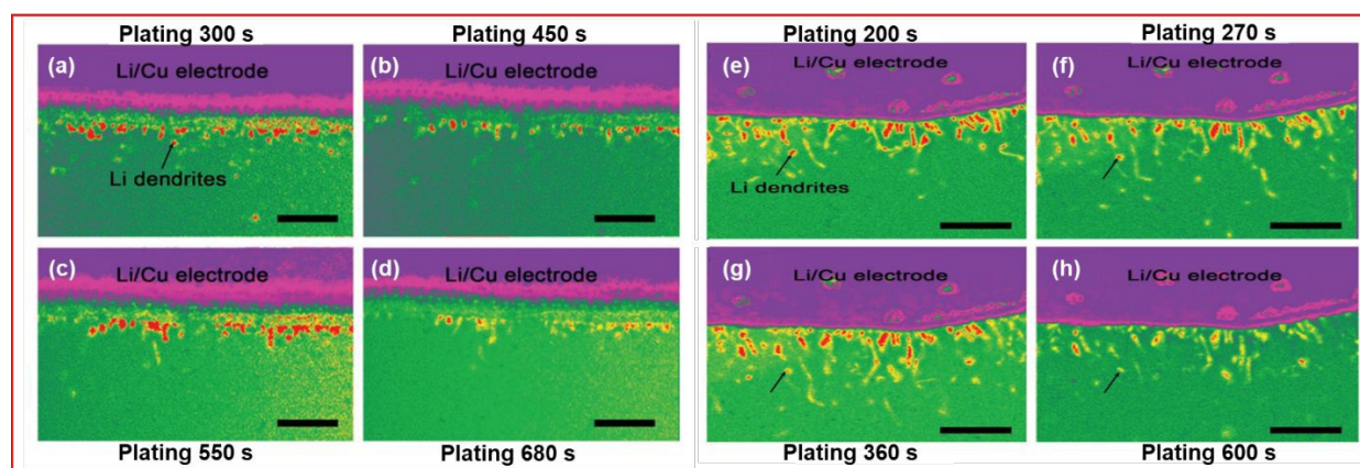
Fig. 13 Operando SEM images of the Li/Cu anode used by Rong et al. at increasing plating times for a solution containing (a-d) 0.2 M \text{Li}_2\text{S}_8 and (e-h) 0.2 M \text{Li}_2\text{S}_8 with 1% wt. \text{LiNO}_3 . Scale bar: 10 \mu\text{m} ((a-h) Adapted with permission from ref. 135, Copyright (2017) Wiley-VCH).
