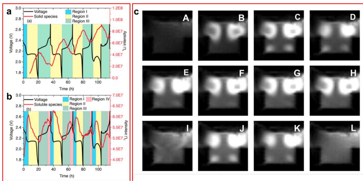
Fig. 5 (a-b) Discharge profile overlapped with ^7\text{Li} NMR spectroscopic data for (a) the insoluble LiPS species and (b) the soluble LiPS species. Where multiple regions are identified, I the initial SEI layer formation phase, II discharging region, III charging region, IV formation of elemental sulfur; (c) ^1\text{H} MRI of an LSB with TEGDME electrolyte. White spots indicate presence of LiPS species. (A) taken at open circuit voltage. (B-H) taken as voltage decreases throughout the discharge and (I-L) as voltage increases throughout the charge process. ((a-b) Reproduced with permission from ref. 75, Copyright (2017) American Chemical Society; (c) Reproduced with permission from ref. 77, Copyright (2022) Elsevier).
