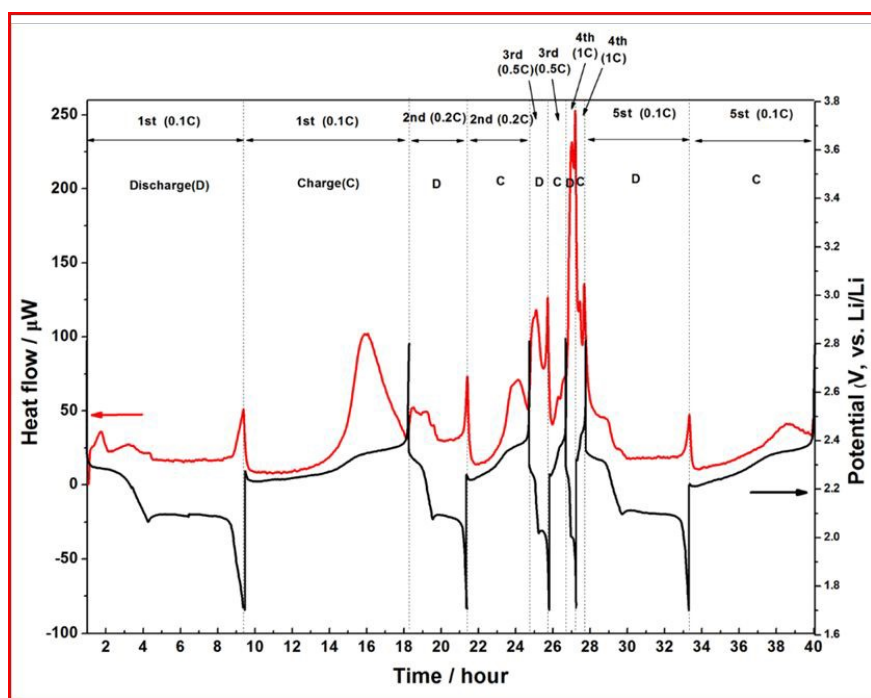
Fig. 16 Discharge profile (black) and heat generation (red) at different C-rates (0.1 C to 1 C) for a nitrogen and phosphorus doped carbon-sulfur cathode. Reproduced with permission from ref. 98, Copyright (2023) Royal Society of Chemistry.
