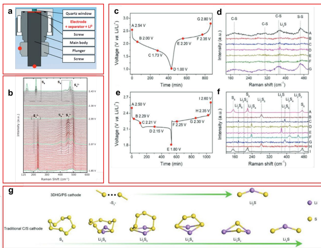
Fig. 3 (a) Schematic of operando Raman cell used for LSB testing; (b) Raman spectra taken at different voltages to monitor the speciation of LiPS with peak labels for specific species; (c-d) Discharge profile (c) and Raman spectra (d) of LSB containing binder-free graphene/polyacrylonitrile sulfur cathode; (e-f) Discharge profile (e) and Raman spectra (f) of LSB containing traditional C-S cathode; (g) Proposed new mechanism of discharge observed with a graphene/polyacrylonitrile sulfur cathode (top) and a traditional C-S cathode (bottom). ((a) Reproduced with permission from ref. 47, Copyright (2015) Wiley-VCH; (b) Reproduced with permission from ref. 43, Copyright (2017) IOP Publishing Limited; (c-g) Adapted with permission from ref. 44, Copyright (2021) Wiley-VCH).
