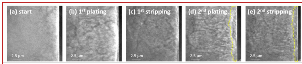
Fig. 11 (a-e) Operando TXM images of the lithium anode morphology on the copper substrate in a \text{Li}_2\text{S}||\text{Cu} cell at 1.5 \text{ mA cm}^{-2} . Yellow line highlights a dense lithium layer formed attributed to SEI layer formation. ((a-e) Adapted with permission from ref. 128, Copyright (2023) American Chemical Society).
