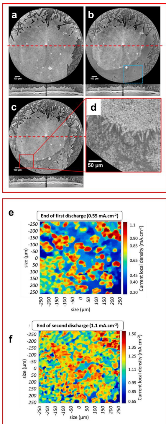
Fig. 9 (a-d) Lateral and transversal XCT images of the cathode at (a) 0% Discharge, (b) 100% Discharge, (c) 100% Charge with (d) an enlarged image of (c). The horizontal red line represents transverse image location. (e-f) 2D images of lithium-electrolyte interface from XCT data at (e) end of 1 st discharge and (f) end of 2 nd discharge. ((a-d) Reproduced with permission from ref. 112, Copyright (2020) American Chemical Society; (e-f) Reproduced with permission from ref. 119, Copyright (2020) Elsevier).
