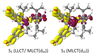
Fig. 11 Difference densities (isovalue \pm 0.002 ) of the S_1 (LLCT/MLCT( d_{xz} )) and S_3 (MLCT( d_{yz} )) states of 3b at the optimized S_0 geometry. Red colour signals electron loss, yellow colour electron gain with respect to the electronic ground state density.
