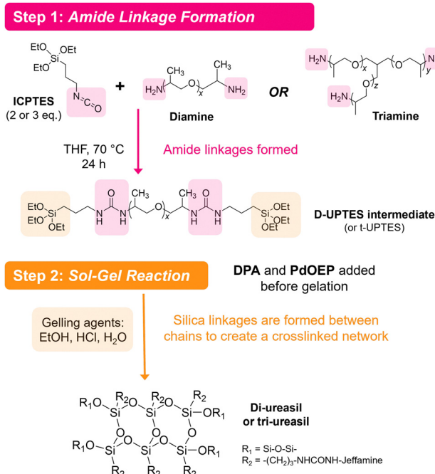
Fig. 2 Reaction scheme for solid-state TTA-UC emitters based on ureasils. Two possible polyetheramine precursor branching structures are shown which yield the four ureasils studied - one lower and one higher molecular weight for each. The sensitizer PdOEP and emitter DPA are mixed with the intermediate before sol-gelation.
