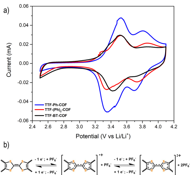
Fig. 5 (a) Cyclic voltammetry of TTF-Ph-COF , TTF-(Ph) 2 -COF , and TTF-BT-COF using 1 M \text{LiPF}_6 in EC/DMC (3/7 v/v) at a scan rate of 0.1 \text{ mV s}^{-1} . (b) Redox mechanism of the p-type TTF moiety in TTF-COFs.
