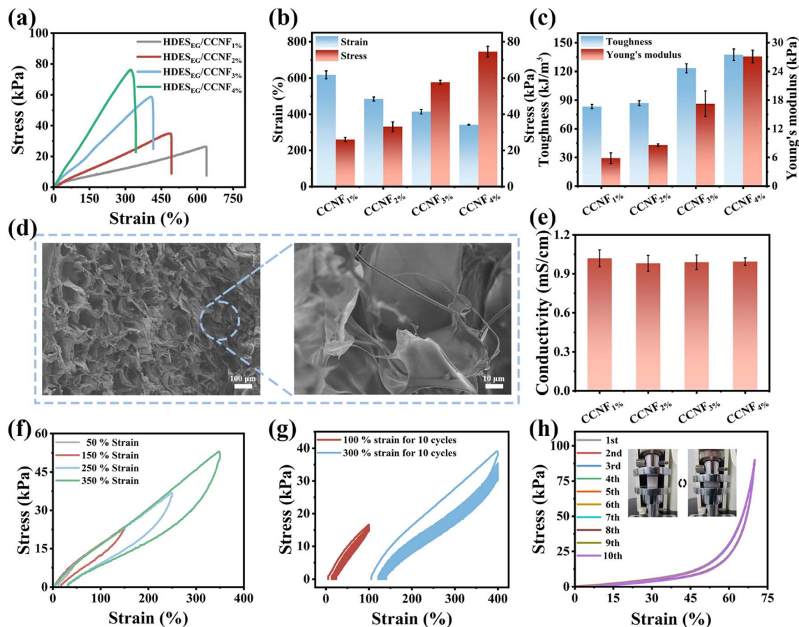
Fig. 3 (a) Stress–strain curves of the four HDES EG /CCNF n hydrogels ( n = 1, 2, 3, 4 ). (b) Strain and stress of HDES EG /CCNF n ( n = 1, 2, 3, 4 ). (c) Toughness and Young's modulus of HDES EG /CCNF n ( n = 1, 2, 3, 4 ). (d) SEM image of HDES EG /CCNF 3% under different magnifications. (e) Conductivity of HDES EG /CCNF n hydrogels ( n = 1, 2, 3, 4 ). (f) Single loading–unloading cycle curves of HDES EG /CCNF 3% hydrogels under different strains (50%, 150%, 250%, and 350%). (g) 10 cycles of loading–unloading curves of HDES EG /CCNF 3% hydrogels without time interval at the strains of 100% and 300%. (h) Schematic diagram and compressive strength of 10 cycles of compression recovery of HDES EG /CCNF 3% hydrogels at a strain of 70%.
