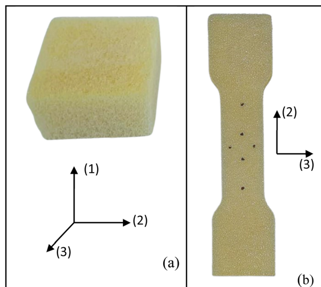
Fig. 2 Compressive (a) and tensile (b) foam samples.
