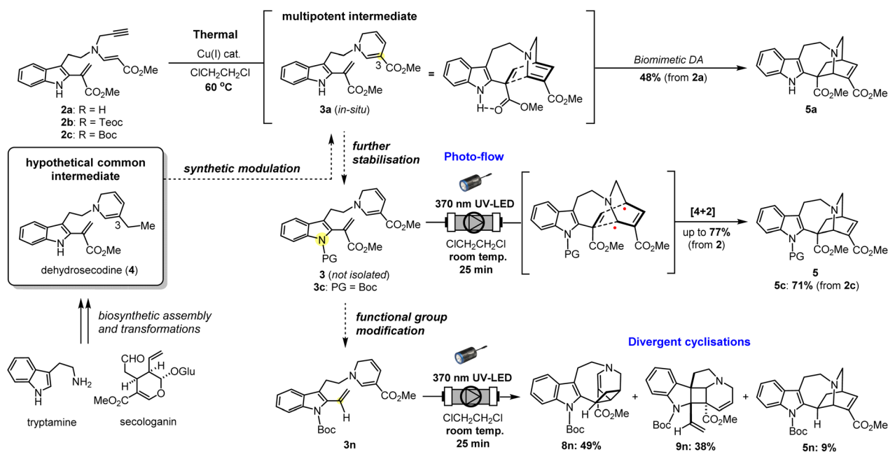
Fig. 7 Biosynthesis of dehydrosecodine (4) initiates from tryptamine and secologanin as building blocks. The thermal biomimetic [4 + 2] cycloaddition proceeds via a dehydrosecodine-type multipotent intermediate ( 3a → 5a ) facilitated by both heating and an intramolecular hydrogen-bonding. The new photo-flow approach features site-selective activation of DHP moiety using stabilised substrates 3 with indole N1 protection. A biradical reaction pathway enabled the divergent [4 + 2] and [2 + 2] cyclisations with minimal conformational changes in the pre-organised structures of 3c and 3n , respectively.
