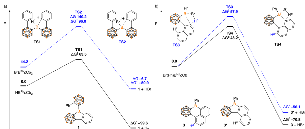
Fig. 5 Energy profile calculated for the conversion of (a) HB^{Ph}OCb_2 and BrB^{Ph}OCb_2 to 1 , and (b) Br(Ph)B^{1Np}OCb to 3 and 3' (in kJ mol ^{-1} ).
