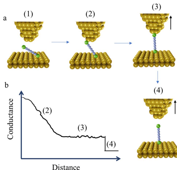
Fig. 3 Schematic illustration of the I (s) or “soft tapping” technique: (a) the steps of molecular junction formation (in this technique molecular junctions are formed without first forming a tip-to-substrate contact); (b) typical conductance–distance trace of the “soft tapping” STM-BJ technique, annotated to illustrate the steps of molecular junction formation.
