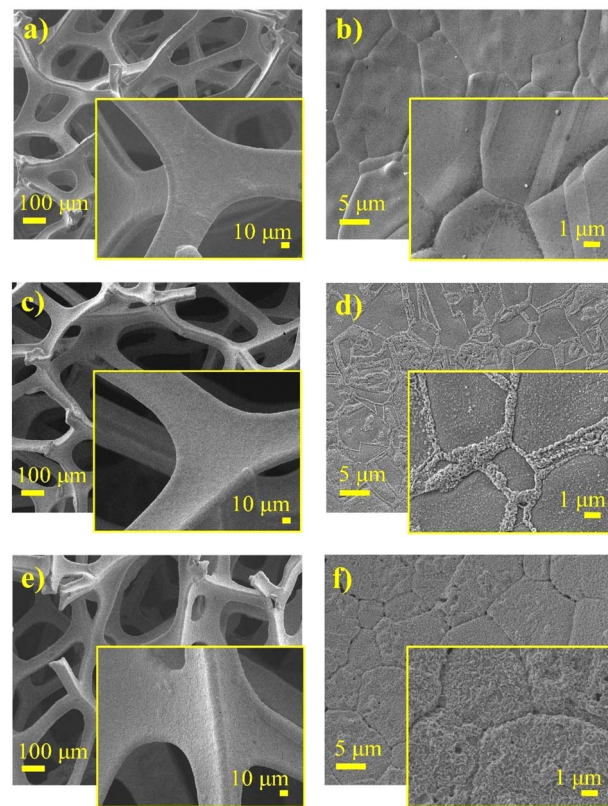
Fig. 3 SEM images of (a and b) \text{Ni} foam, (c and d) \text{NiO@Ni} foam, and (e and f) \text{C@NiO@Ni} foam.
