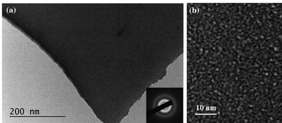
Fig. 1 TEM images and SAED pattern (inset) of dense Ta 2 O 5 films at different magnifications (a) 40 000 \times and (b) 150 000 \times (Reproduced from ref. 43 with permission from Springer Nature copyright [2024]).
