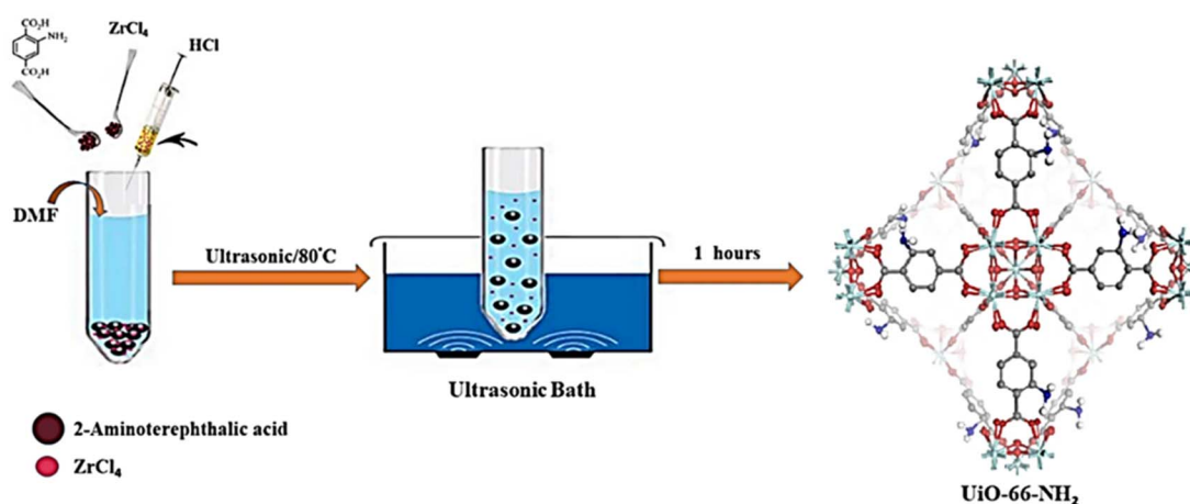
Fig. 9 UiO-66- \text{NH}_2 synthesized via a novel sonochemical method. Adopted with permission from ref. 71 Copyright (2023) Scientific Reports.
