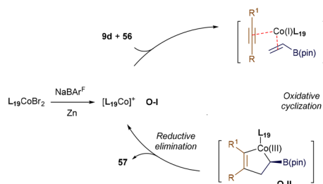
Scheme 21 Co(I)-catalyzed [2 + 2] cycloaddition.
