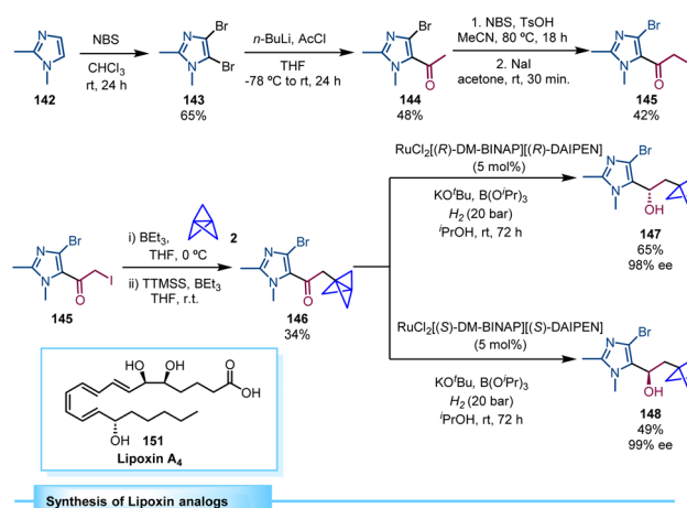
Synthesis of Lipoxin analogs
