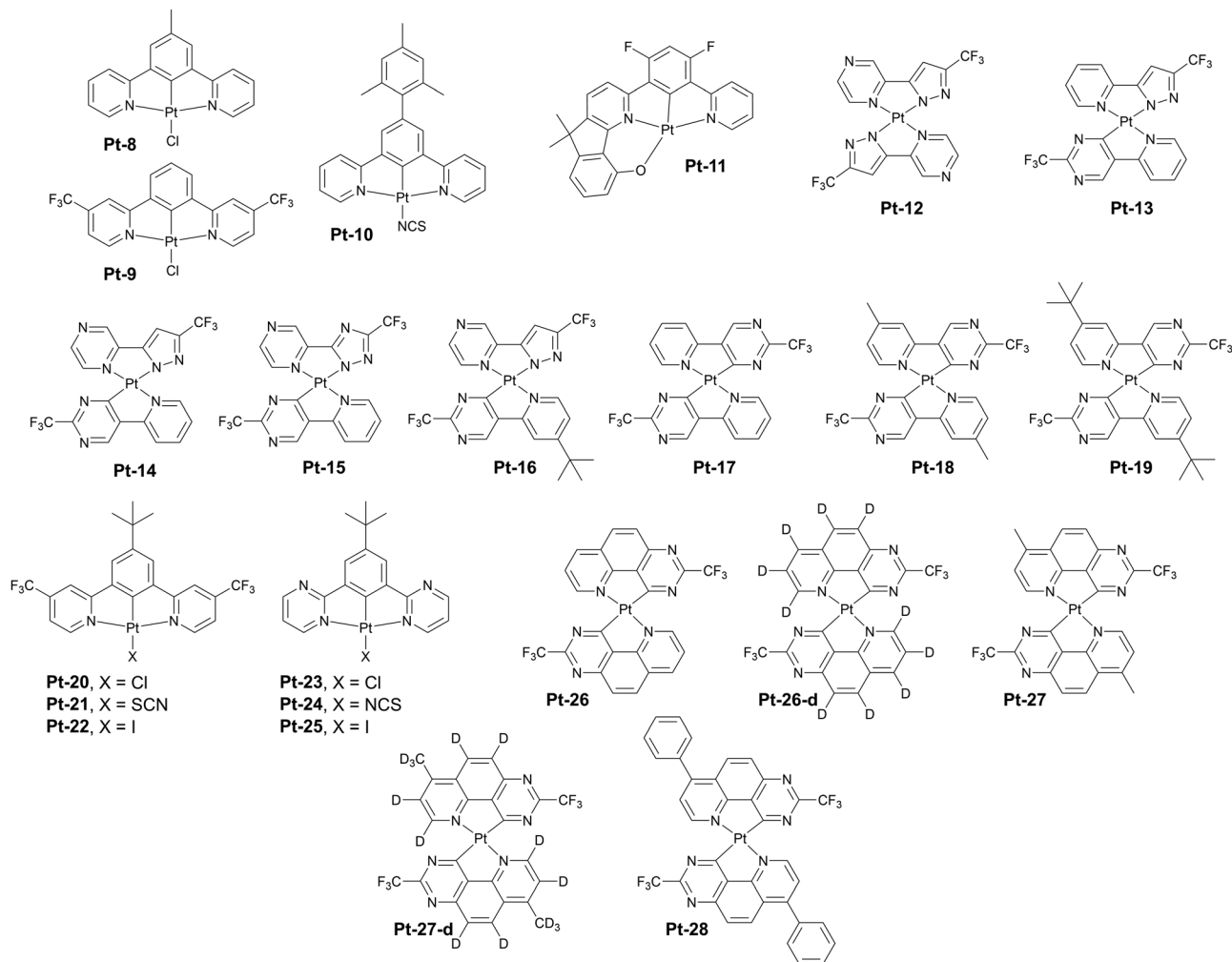
Fig. 9 Examples of aggregating platinum(II) complexes with long wavelength NIR photo- and electrochromism in neat films.
