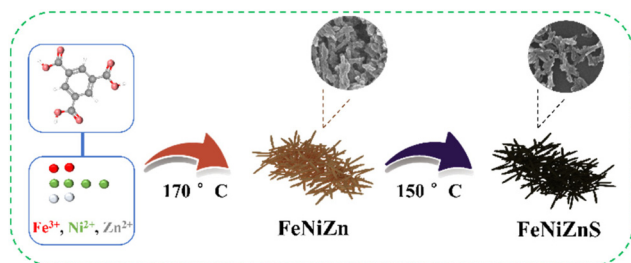
Scheme 1 The synthetic procedures of the trimetallic MOF template and FeNiZnS catalysts.
